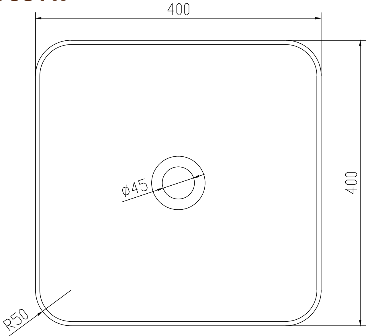
290090 Solidthin-QR L400xW400xH125mm
